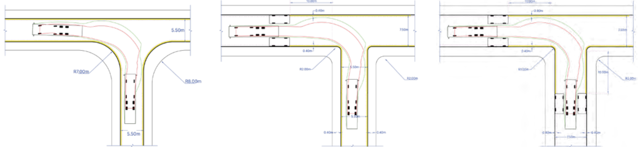
Diagrams for Table B: Kerb Radii for Local Street/ Local Street junctions
